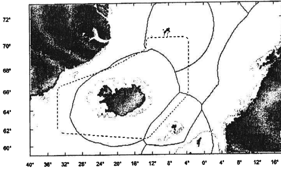
Proposed survey area for cruise A7/12/ 4 July-15 August 2012 (broken line).
