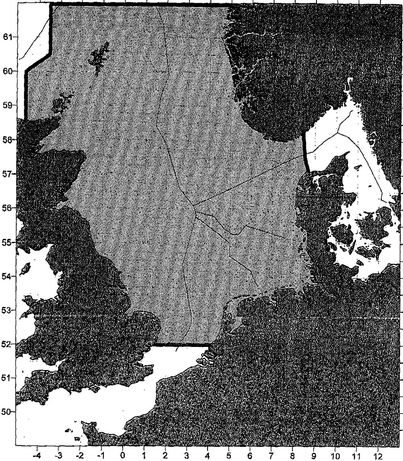
North Sea acoustic survey for herring, TRIDENS 23 June - 17 July 2008 The outer border of the survey area is indicated in black.
