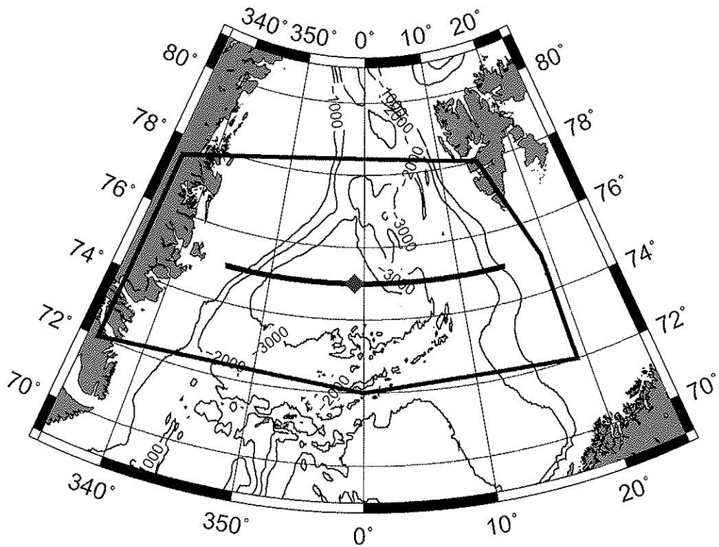
Working area and main transect Polarstern 2010, ARK XXV/1
