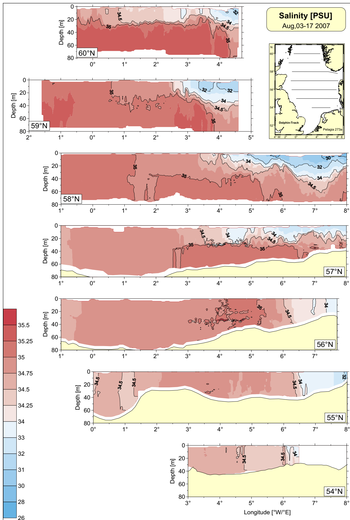
Fig. 2b: Salinity sections measured with the towed Dolphin system (raw data)
