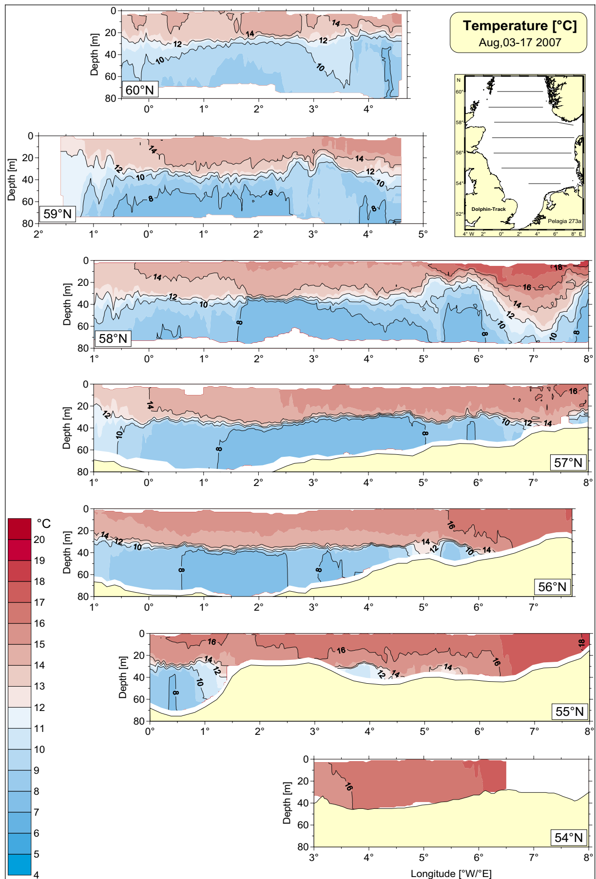
Fig 2a: Temperature sections measures with the towed Delphin system (raw data)
