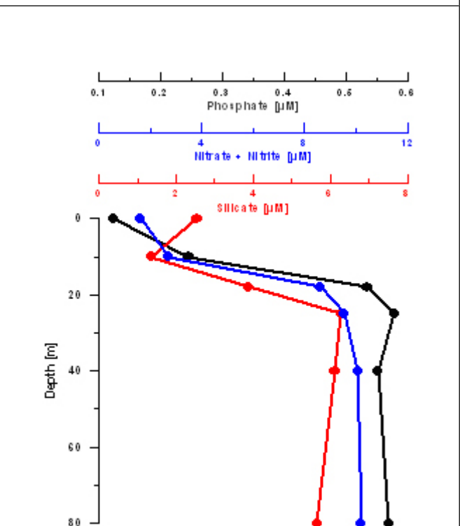
Figure 11. Profiles of inorganic nutrients at station AL275-420-2.
