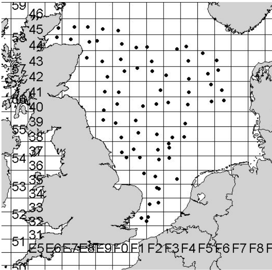
Map of sampling locations.
