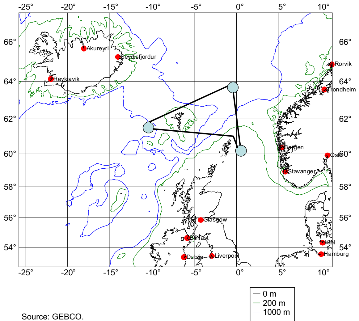
Stations (blue) and transects during the research cruise
