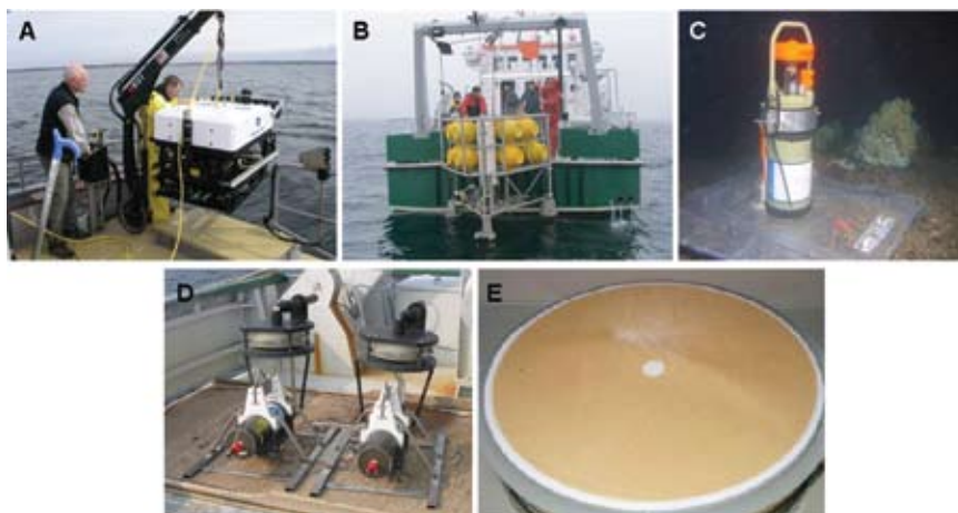
Figure 3. Examples of equipment deployed at the Tisler reef. (A) Remotely operated vehicle. (B) Lander being deployed from support ship R/V Nereus . (C) Recording current meter RCM9. (D) Stand-alone in situ pump (SAPS) in special bottom frame. (E) Loaded SAPS filter.
