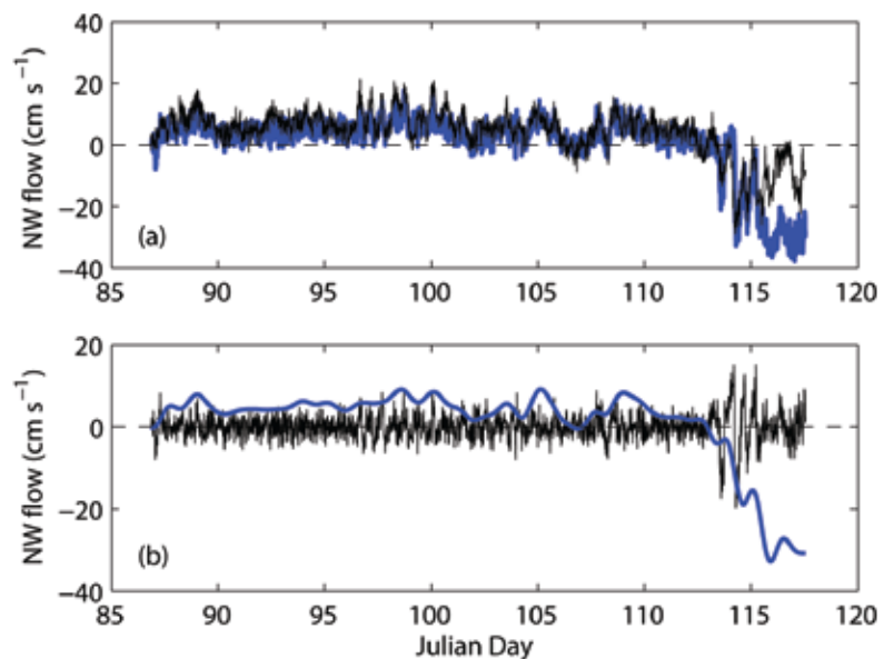
Figure 4. Time series of (a) northwest-directed current at 4 mab (blue) and 24 mab from the spring 2006 LF ADCP deployment at the sill. In (b), the 4-mab data are shown after application of a 27-hr filter for the low (blue) and high (black) components to separate residual and tidally dominated flows.
