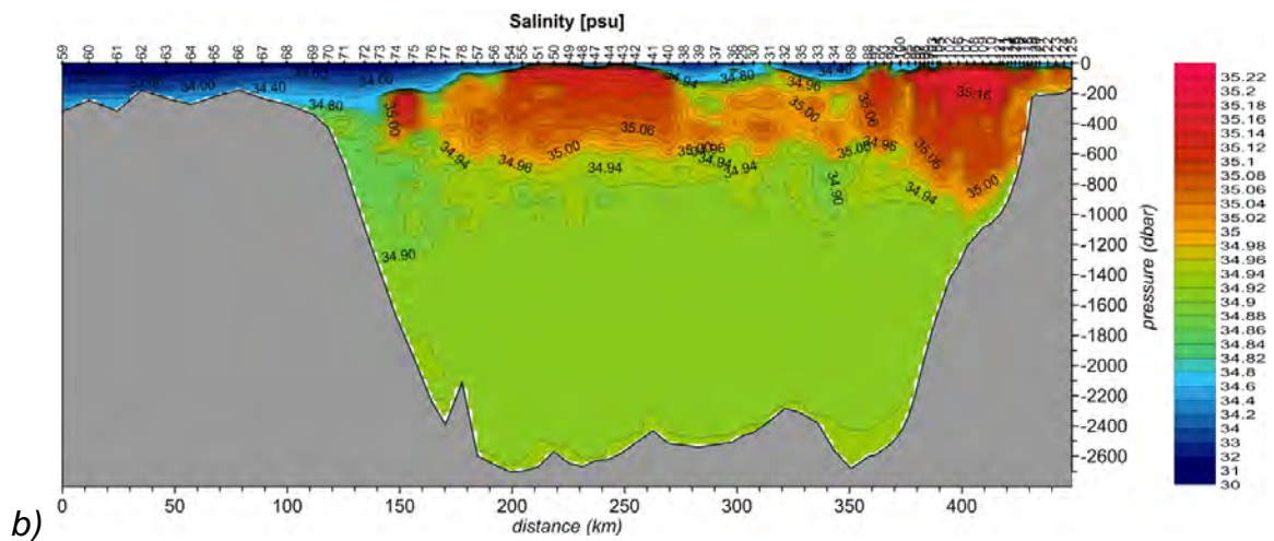
Fig. 3.3: Vertical distribution of potential temperature (a) and salinity (b) at the section across Fram Strait measured during ARKXXVI/1.
