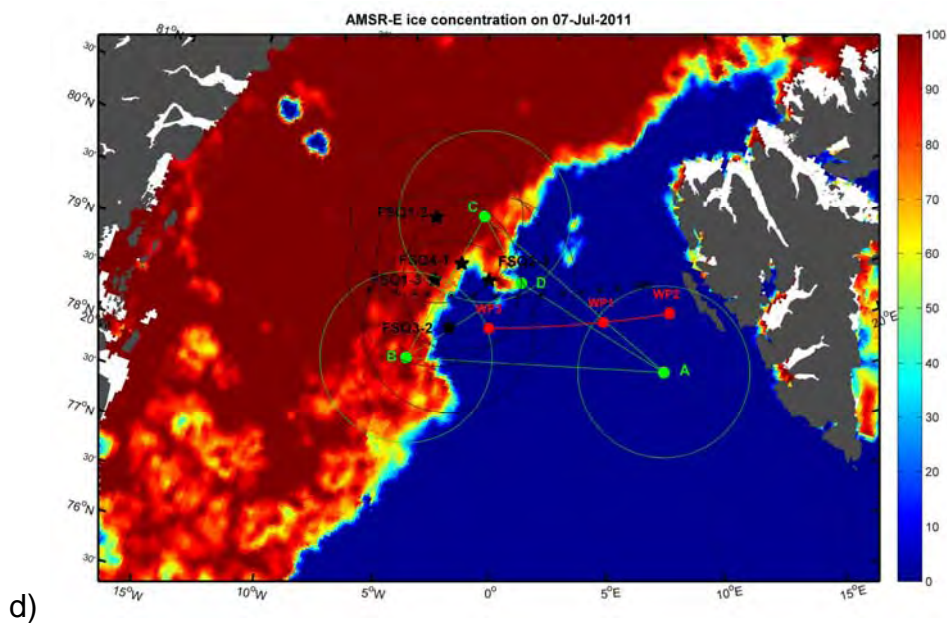
Fig. 3.2: The moored array in Fram Strait: (a) the data quality from recovered instruments, (b) the part of array redeployed in 2011 (marked with a dashed box), (c) a configuration of acoustic modems and (d) positions and nominal ranges of the RAFOS sound sources (black stars) deployed during ARKXXVI/1. The green dots indicate positions of tomographic sources deployed by NERSC in 2010.
