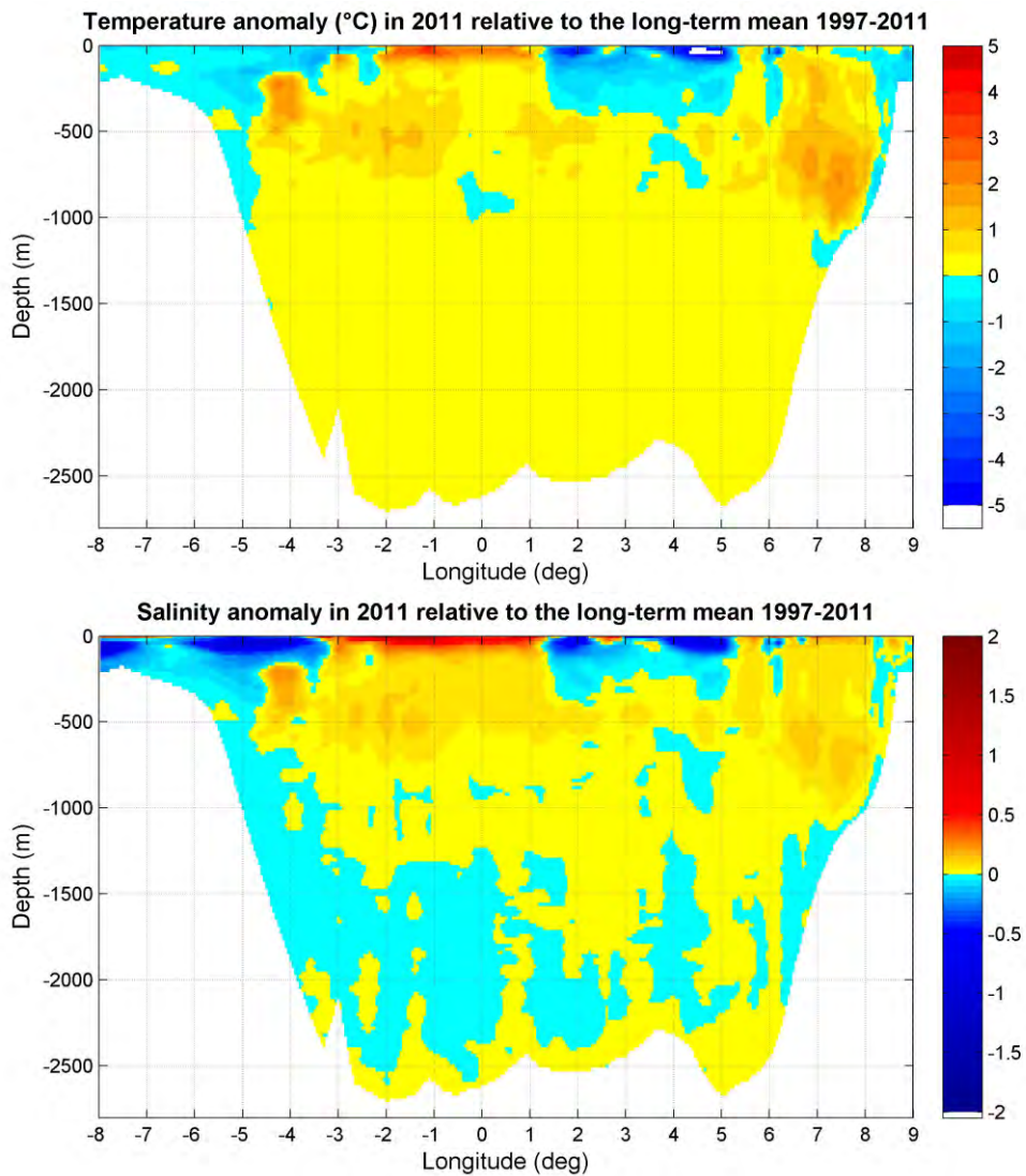
Fig. 3.4: Temperature and salinity anomalies measured in 2011 during ARKXXVI/1 relative to their long-term means (1997-2011).
