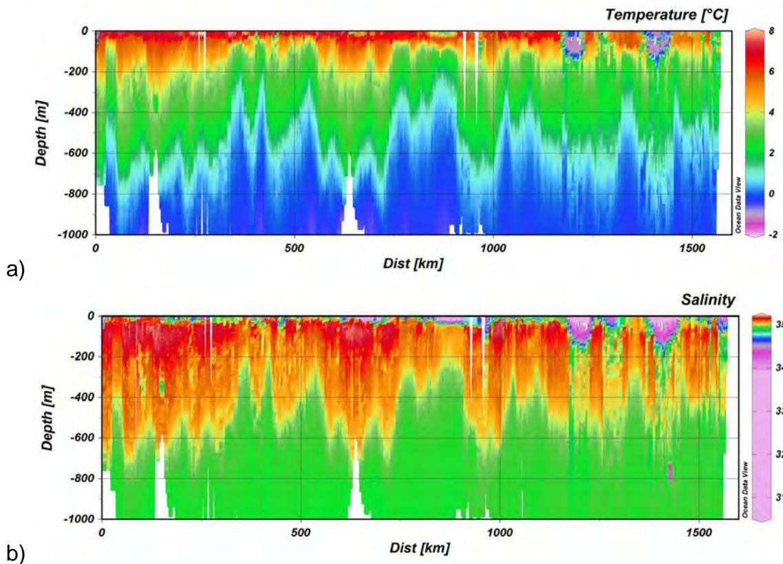
Fig. 3.8: (a) Temperature and (b) salinity measured by the glider SG127 during the total duration of the summer mission 2011.
