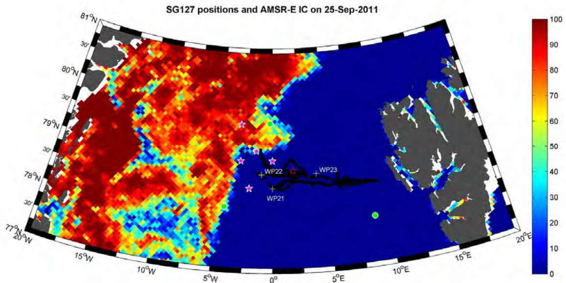
Fig. 3.9: The glider SG127 track shown in relations to the sea ice concentration during the recovery.
