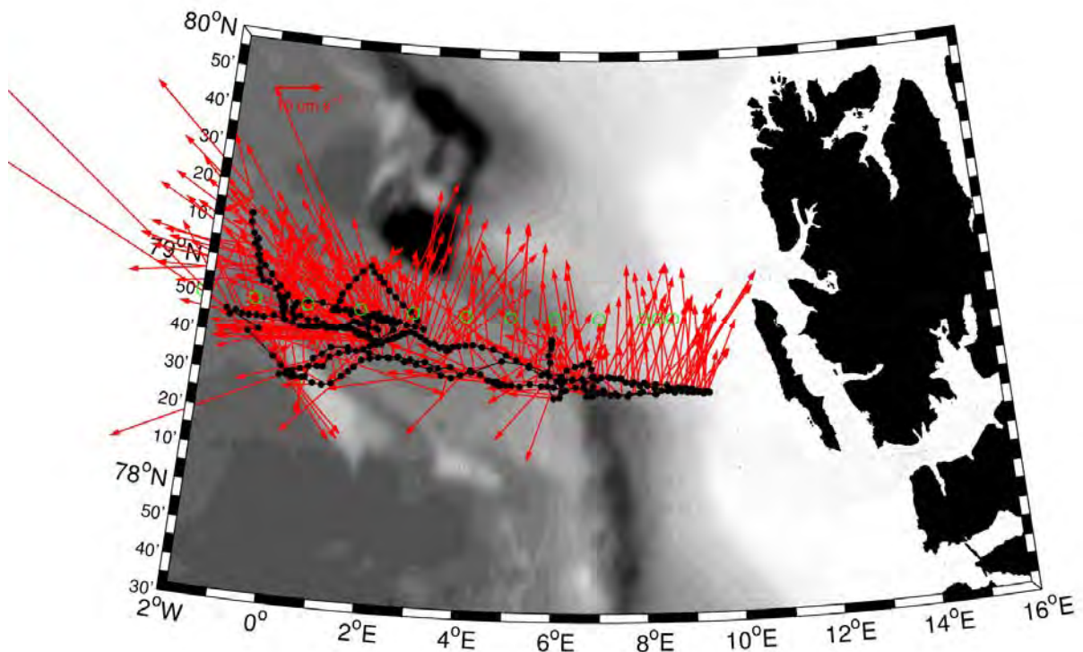
Fig. 3.7: Locations of the Seaglider surfacing positions between successive dives and vertically averaged currents during the summer mission 2011 in the eastern and central Fram Strait from July 9 to September 25.
