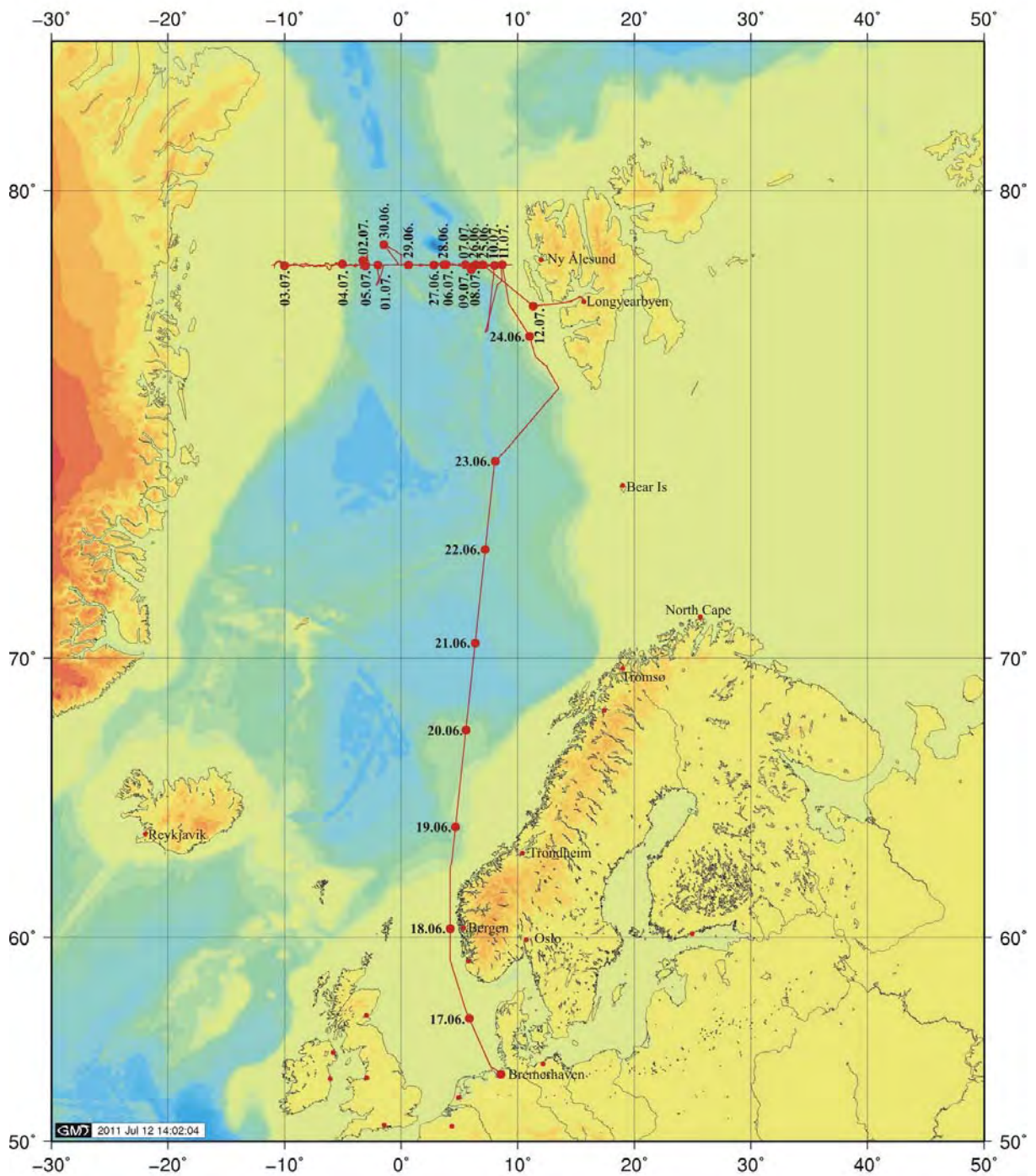
Fig. 1.1: Cruise track of RV Polarstern during the expedition ARK-XXVI/1
