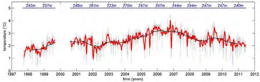
Fig. 3.6: Time series of the Atlantic Water temperature (a) in the West Spitsbergen Current core, (b) at the West Spitsbergen Current western edge and (c) in the AW recirculating branch in 1997-2011, measured by CTD sensors or T sensors at current meters at the nominal depth 250 m.
