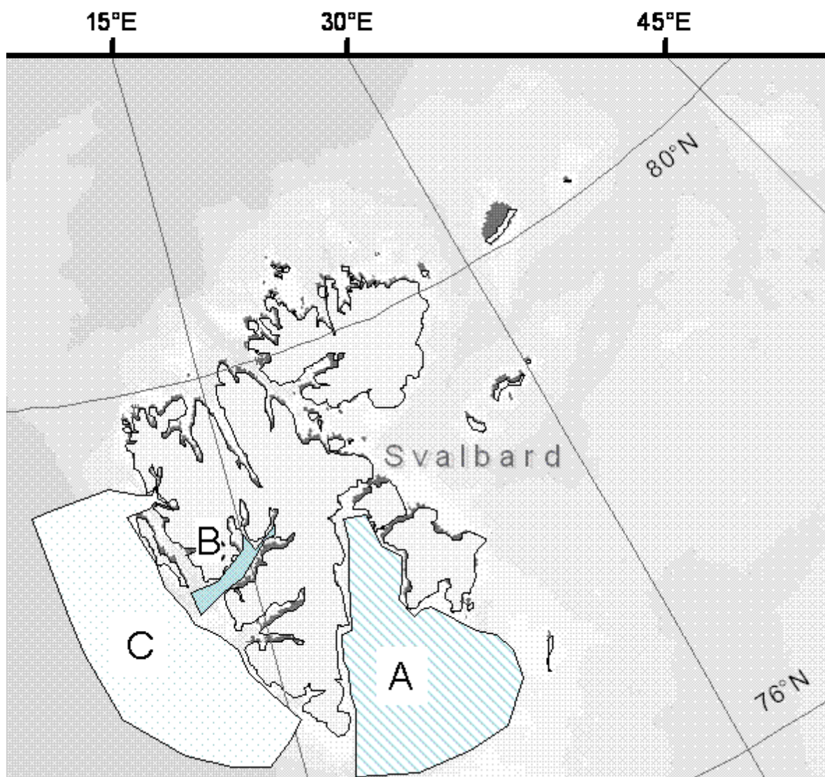
AI-2: Target area A, B, C, the Storfjorden (region A, box centred at 19^{\circ} 40'E , 77^{\circ}00'N ), the Isfjorden (region B, box centred at 78^{\circ} 13' N , 15^{\circ} 38' E ) and the Prins Karls Forland and Kongsfjorden, Ny-Ålesund (region C, box centred at 78^{\circ} 00'N , 11^{\circ} 30'E ). Depend on the ice coverage and sea state water and sediment samples will be gathered.
