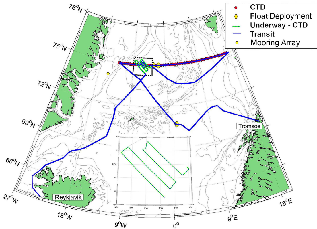
Figure 1: cruise track of RV Poseidon cruise P437-2, August 15 to September 7 2012, with CTD-casts (red dots), Argo float deployments (yellow diamonds) and UCTD-profiles (dashed green-blue line). Enlargement of the UCTD-survey in the lower part of the map.
